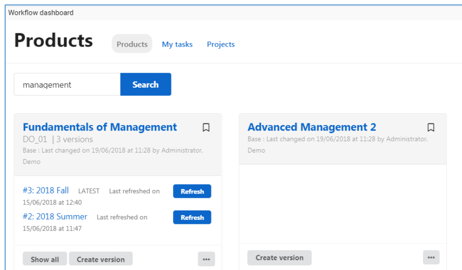
Figure 1 Product dashboard
